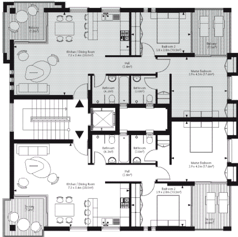
Typical apartment layout
