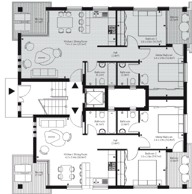
Typical apartment layout
